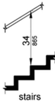
Figure 5 - Handrail Height
