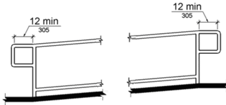
Figure 1 - Top and Bottom Handrail Extension at Ramps
