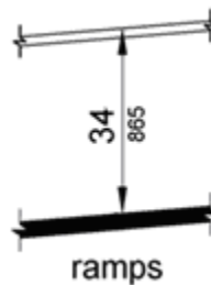
Figure 3 - Handrail Height
